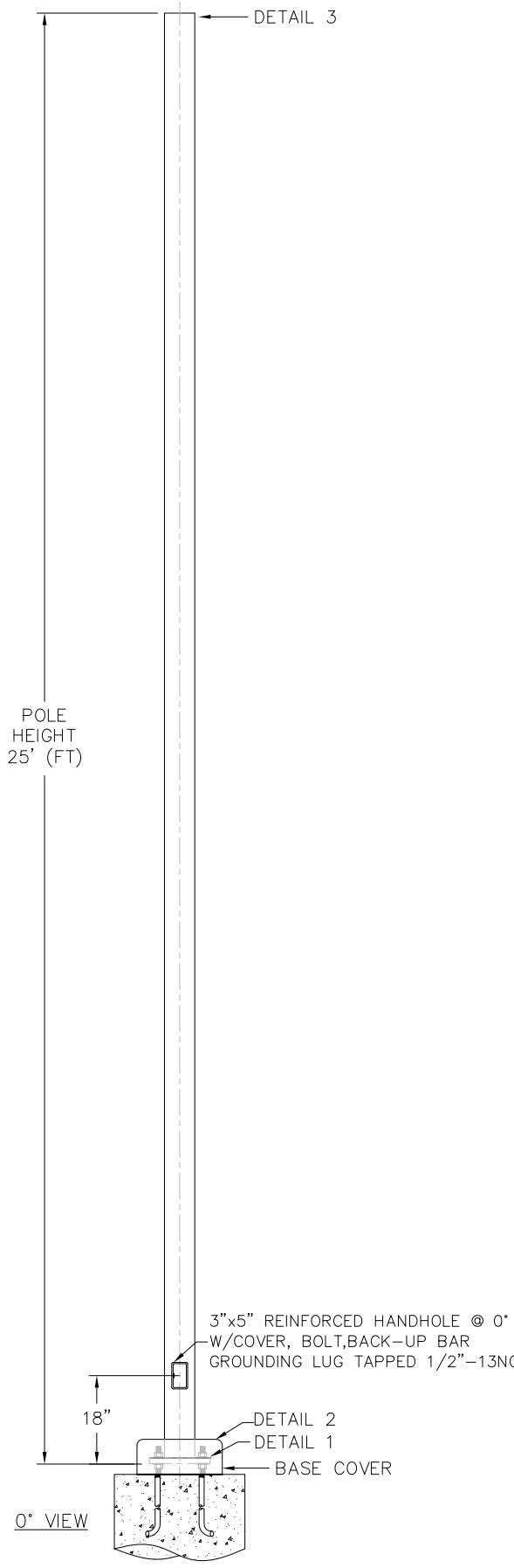
DETAIL 3 POLE TOP | DETAIL 1 BASE PLATE | DETAIL 2 ANCHOR BOLT
