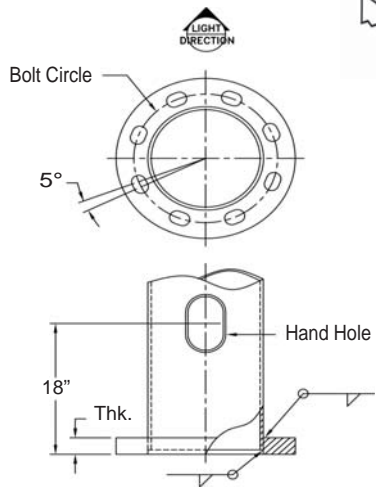
Base Plate Detail
